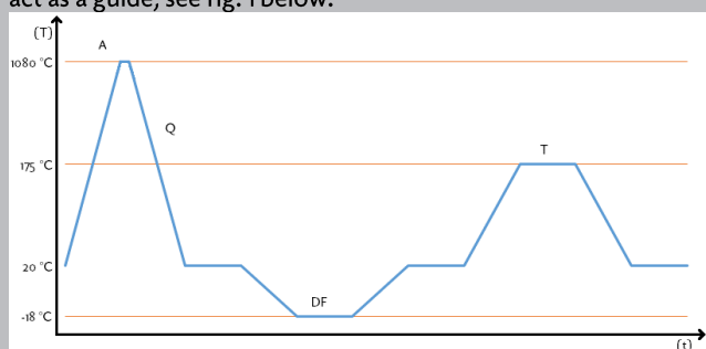
Figure 1: Schematic hardening and tempering curve
